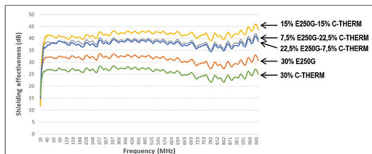
Figure 2: Shielding effectiveness of PP compounds containing different carbon black blends
