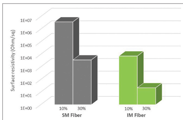
Figure 6: Surface resistivity of PA66 reinforced with 300 micron recycled carbon fibre granulates. Data obtained at 10 and 30 wt% fibre content for standard modulus (SM) and intermediate modulus (IM) grades
